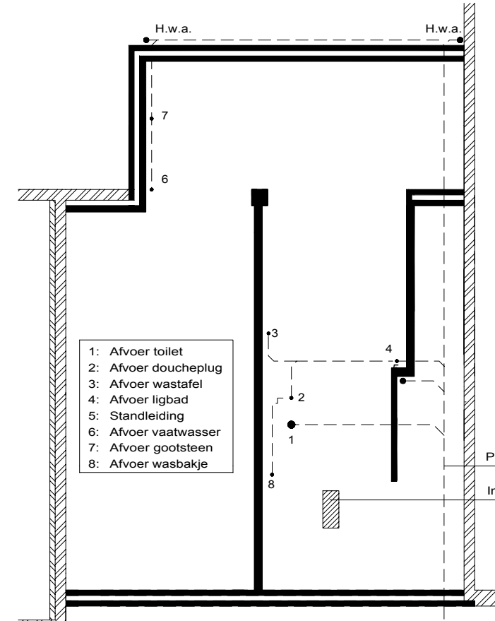
Schema riolering
