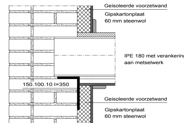
Detail oplegging IPE 180
